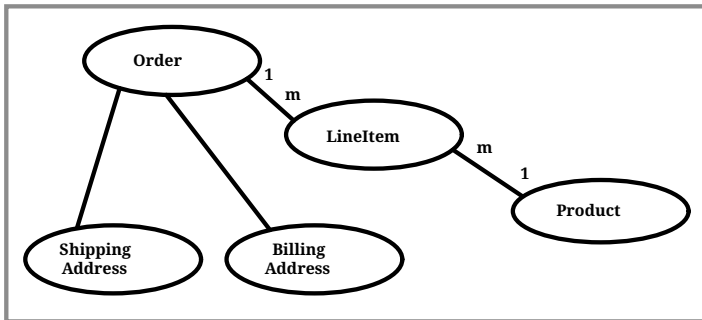
Figure 1. Abstract Persistence Schema of Several Entities with Defined in the Same Persistence Unit.
